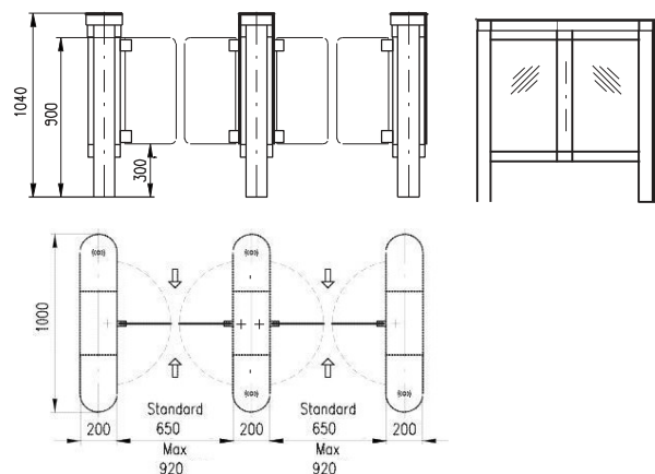
BGI Flap Barrier FP : 40 / FP : 120 - dual barrier panel
