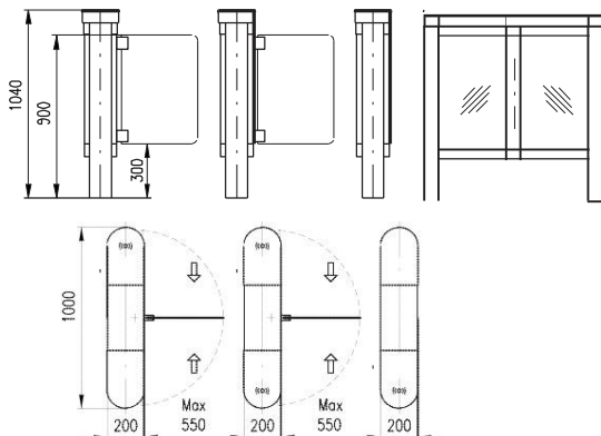
BGI Flap Barrier FP : 40 / FP : 120 - single barrier panel
